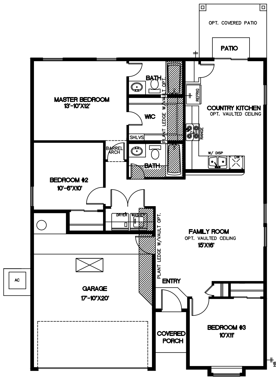
FLOORPLAN
