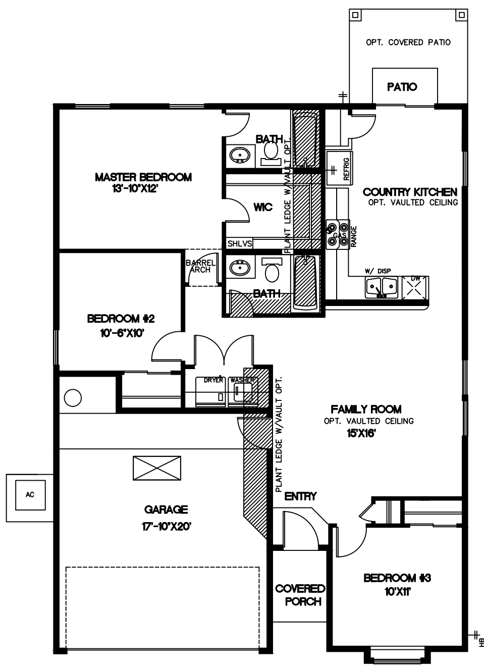
FLOORPLAN
