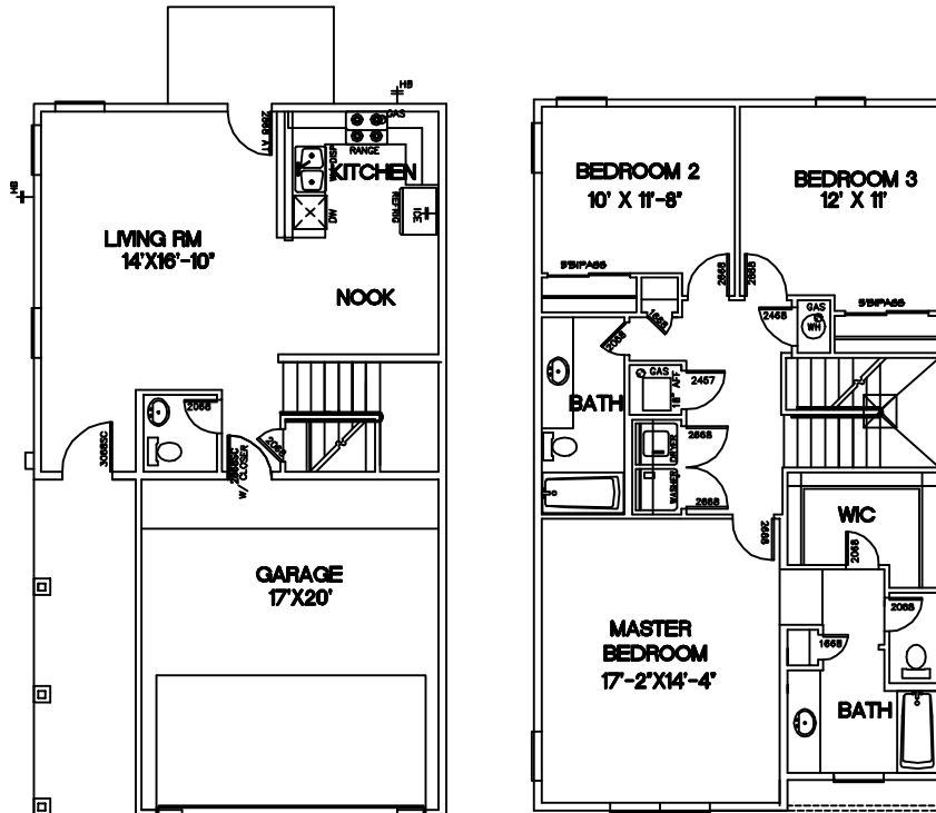
FLOORPLAN
